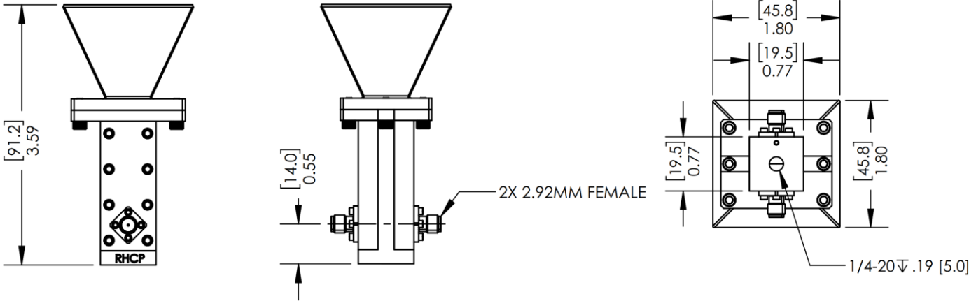
Dimensions shown in inches [millimeters] Tolerances in millimeters - Integer: \pm 3 , One Place Decimal: \pm 0.1 , Two Place Decimal: \pm 0.05
